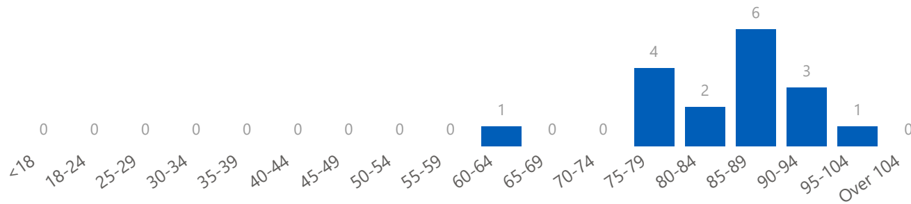
Solihull Hospital Positives - By Age Group, Gender, & Ethnicity
