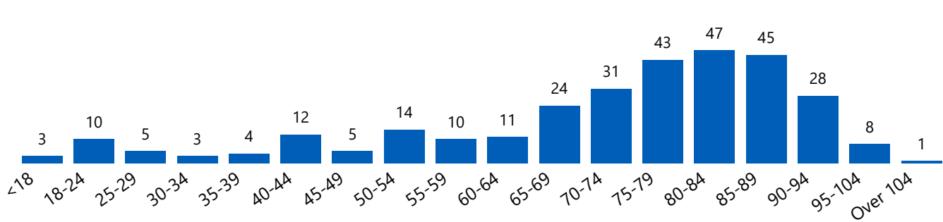
UHB Positives - By Age Group, Gender, & Ethnicity
