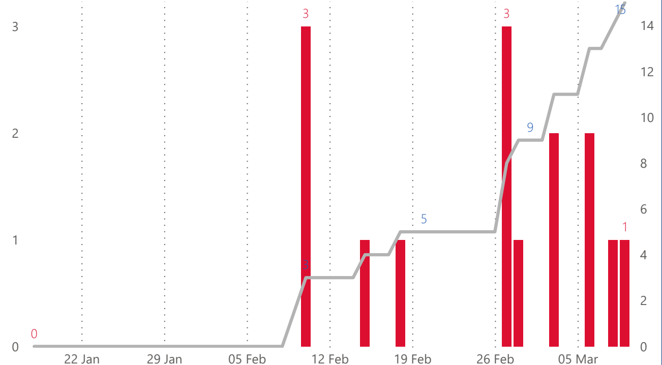
Solihull Hospital - Inpatient - Daily Positives (Bars) & Cumulative (Line)
