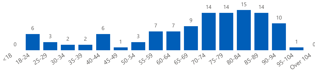
Queen Elizabeth Hospital Positives - By Age Group, Gender, & Ethnicity
