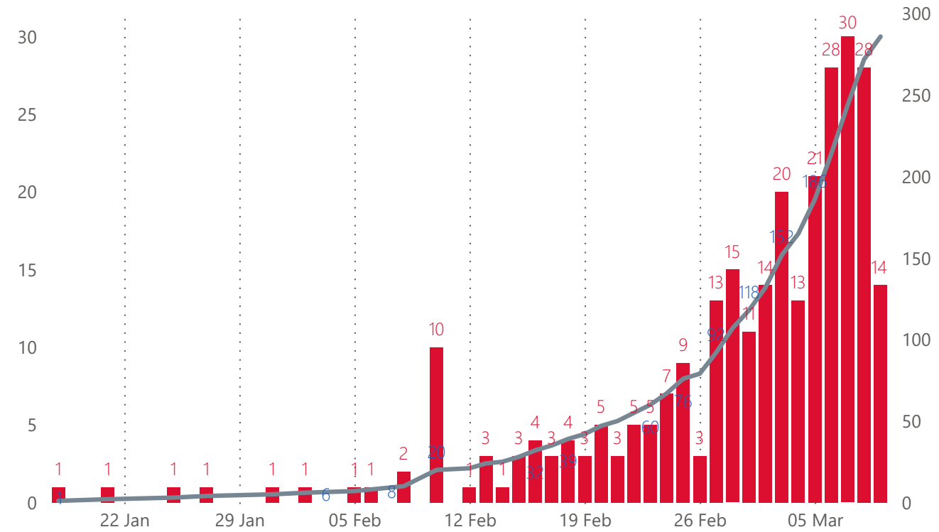
UHB - Inpatient - Daily Positives (Bars) & Cumulative (Line)
