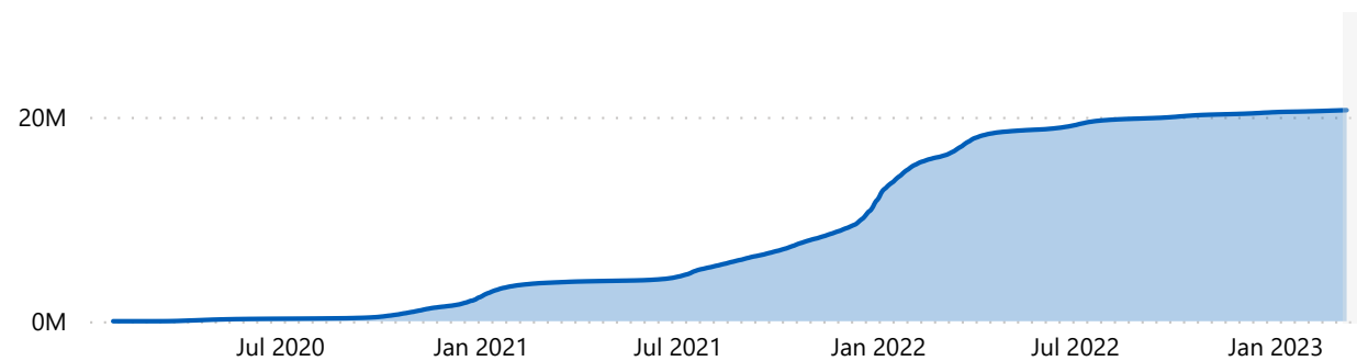
Cumulative cases by specimen date
