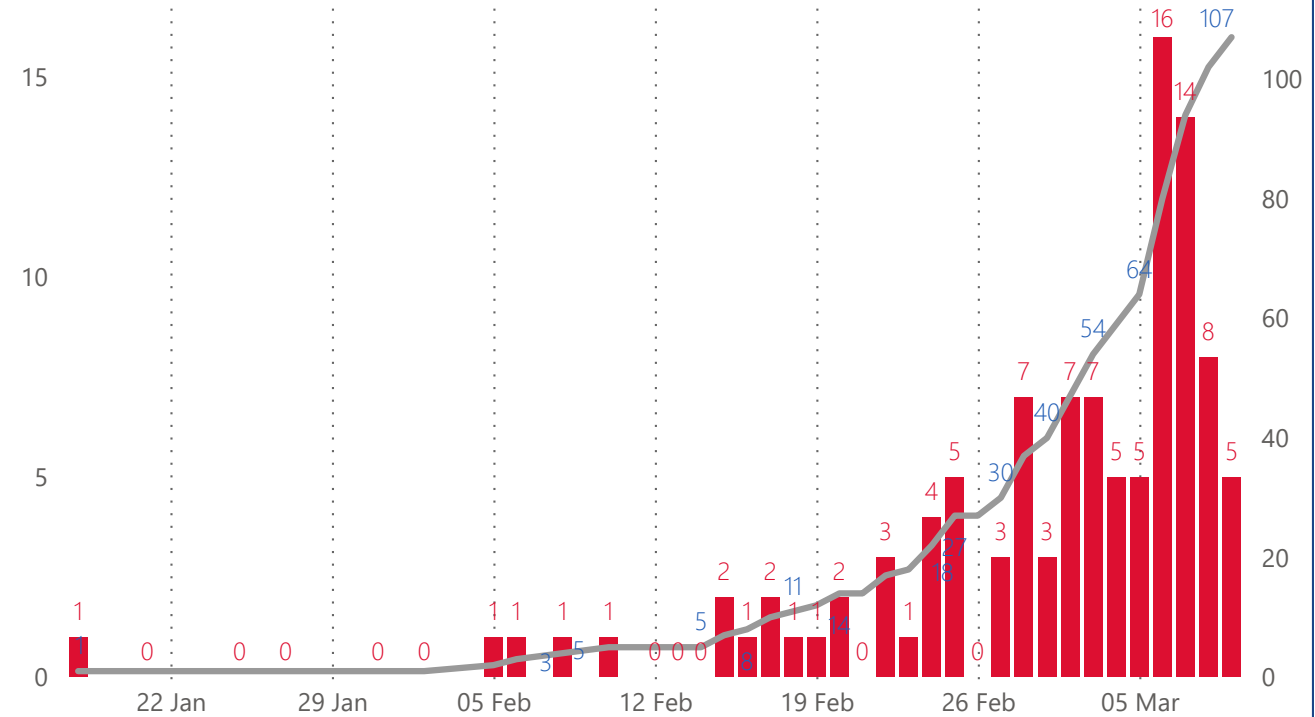
Queen Elizabeth Hospital - Inpatient - Daily Positives (Bars) & Cumulative (Line)
