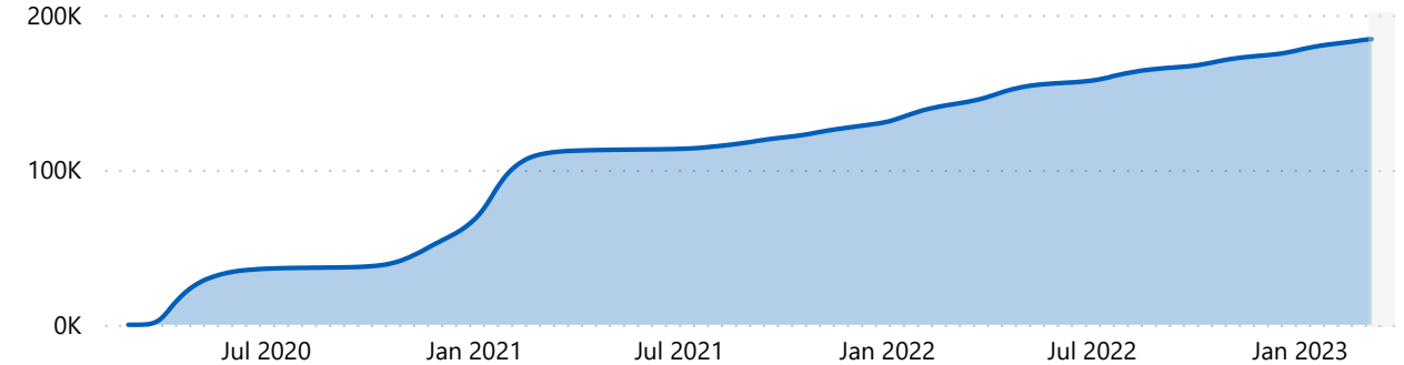
Cumulative deaths by date of death
